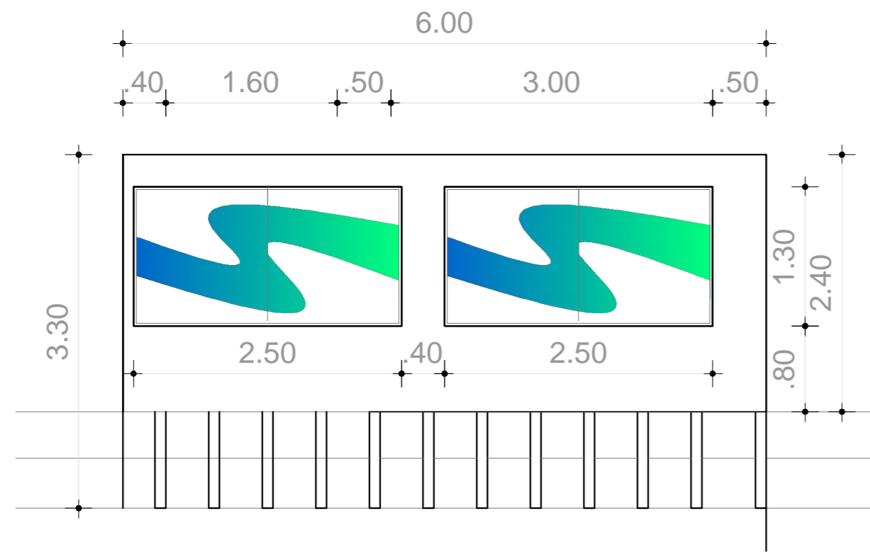
03 Fachada Principal ESC: 1/50
